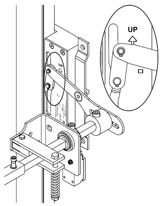
Figure 6: Safety gear position on inverted guide rails
